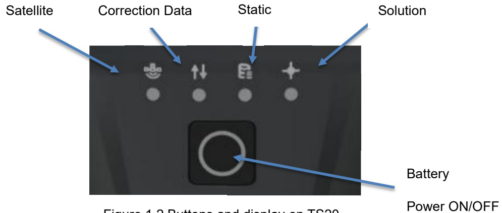
Figure 1.2 Buttons and display on TS20
