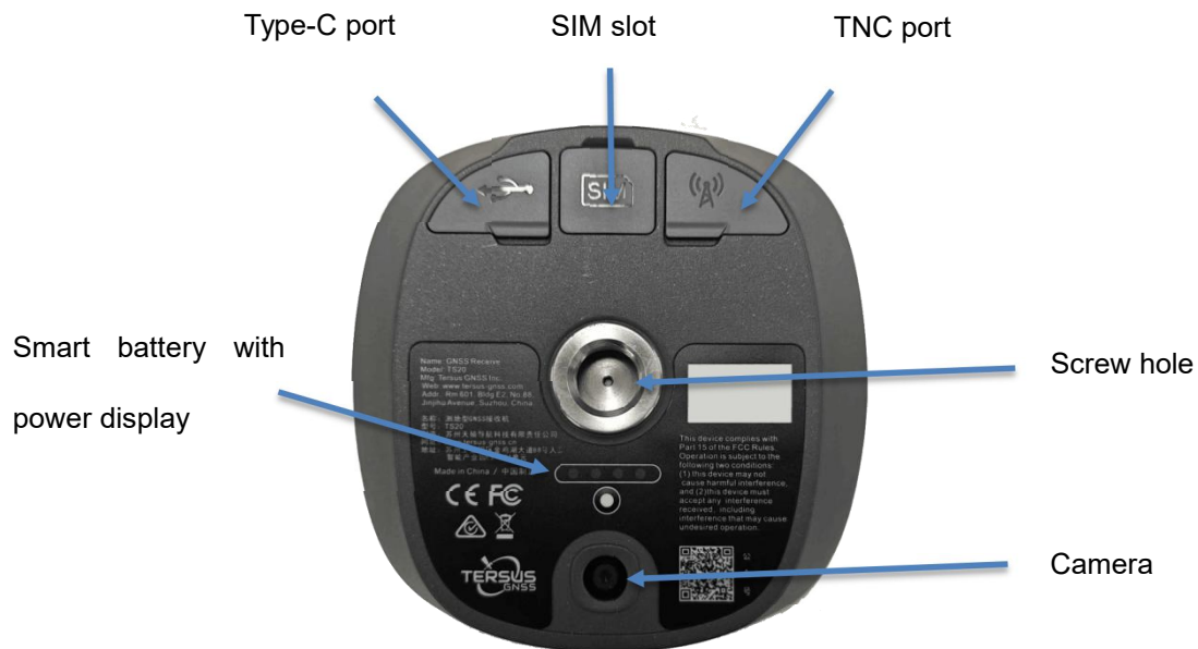
Figure 1.4 Bottom of TS20 GNSS receiver
